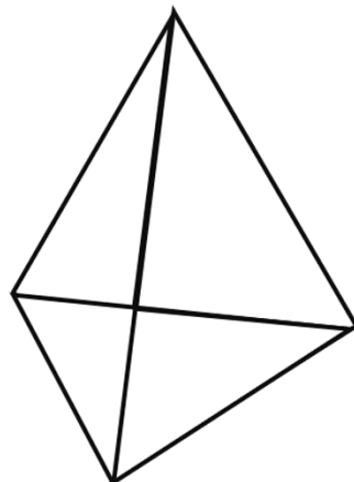
Triangular-based pyramid
