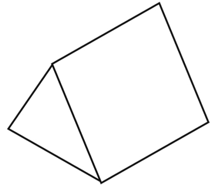
Triangular prism
