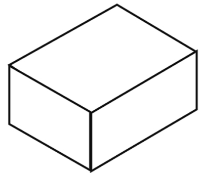
Cuboid
