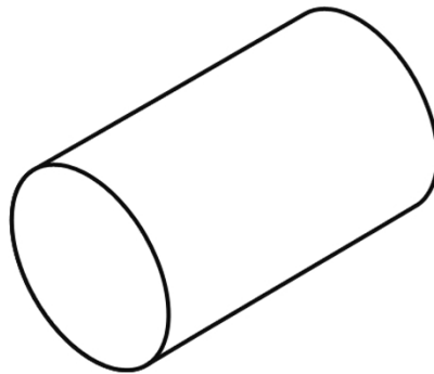
Cylinder
